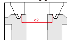
Measure inside diameter of RTJ ring groove
