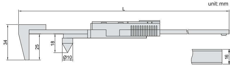
Measure edge to hole center distance
