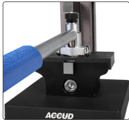
Bore gauge setter for setting zero (optional)
