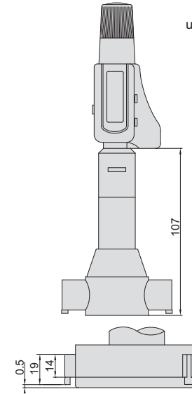
extension rod(included)
