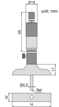
Rod (included)
