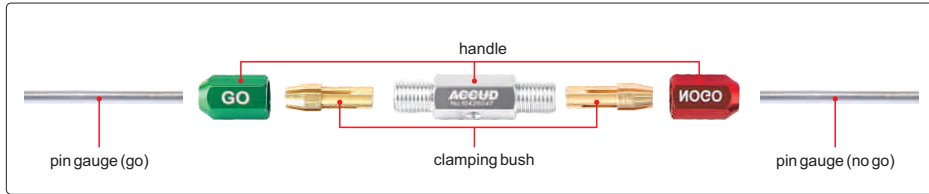
before assemble
