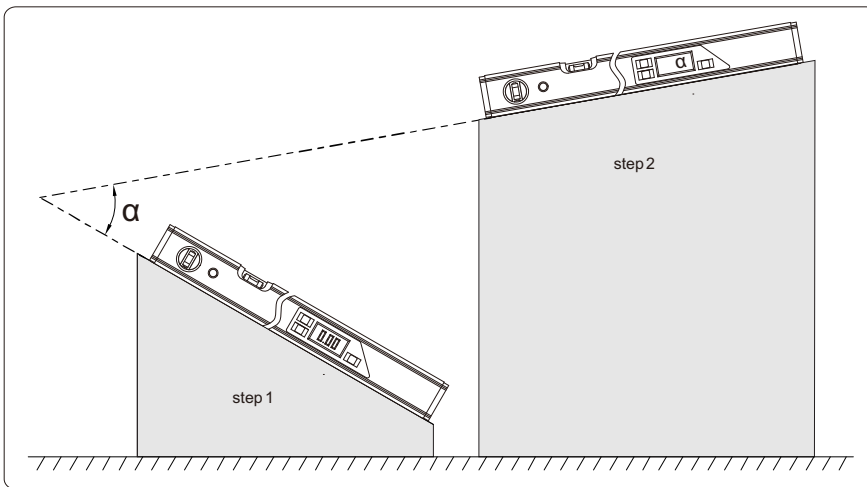
Measure the angle of two separate surfaces
