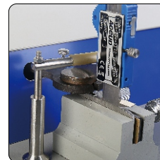
lapping measuring surfaces of caliper lower jaws
