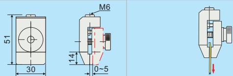
CAM GRIP (Code: DF-CG1)
