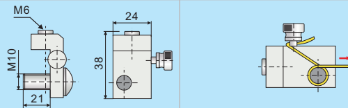
WIRE TERMINAL GRIP (Code: DF-TWG1)
