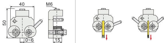
CAM GRIP (Code: DF-CG2)
