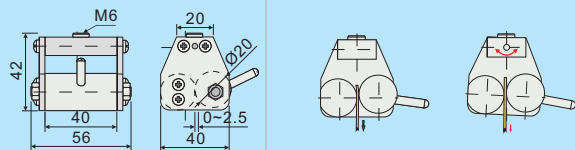
CAM GRIP (Code: DF-CG2)
