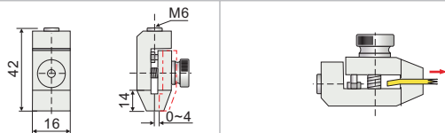
FLAT CHUCK (Code: DF-FC2)
