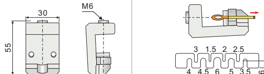
WEDGE GRIP (Code: DF-WT1)
